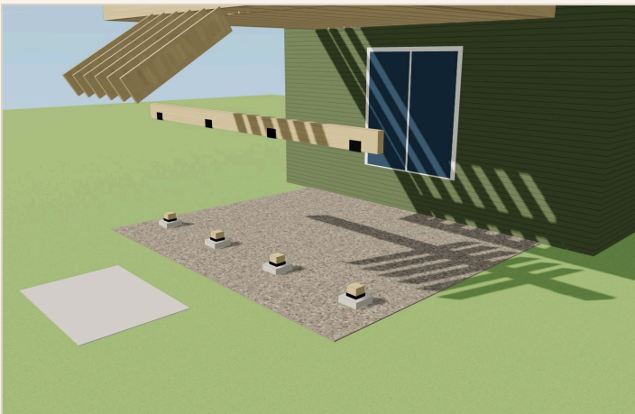
Exploded — from the front corner
