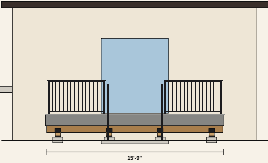
FRONT ELEVATION — from the yard
