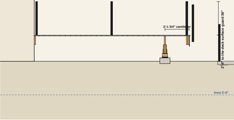
SECTION through zone A at 7'-10 1/2" — looking toward the left end
